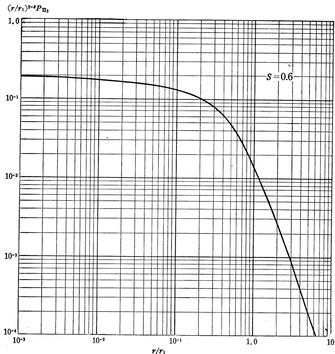
Fig. 2. Normalized Lateral Structure Function for s=0.6 in Approximation B. Molière unit is r_1 = E_s / \epsilon cascade units.
