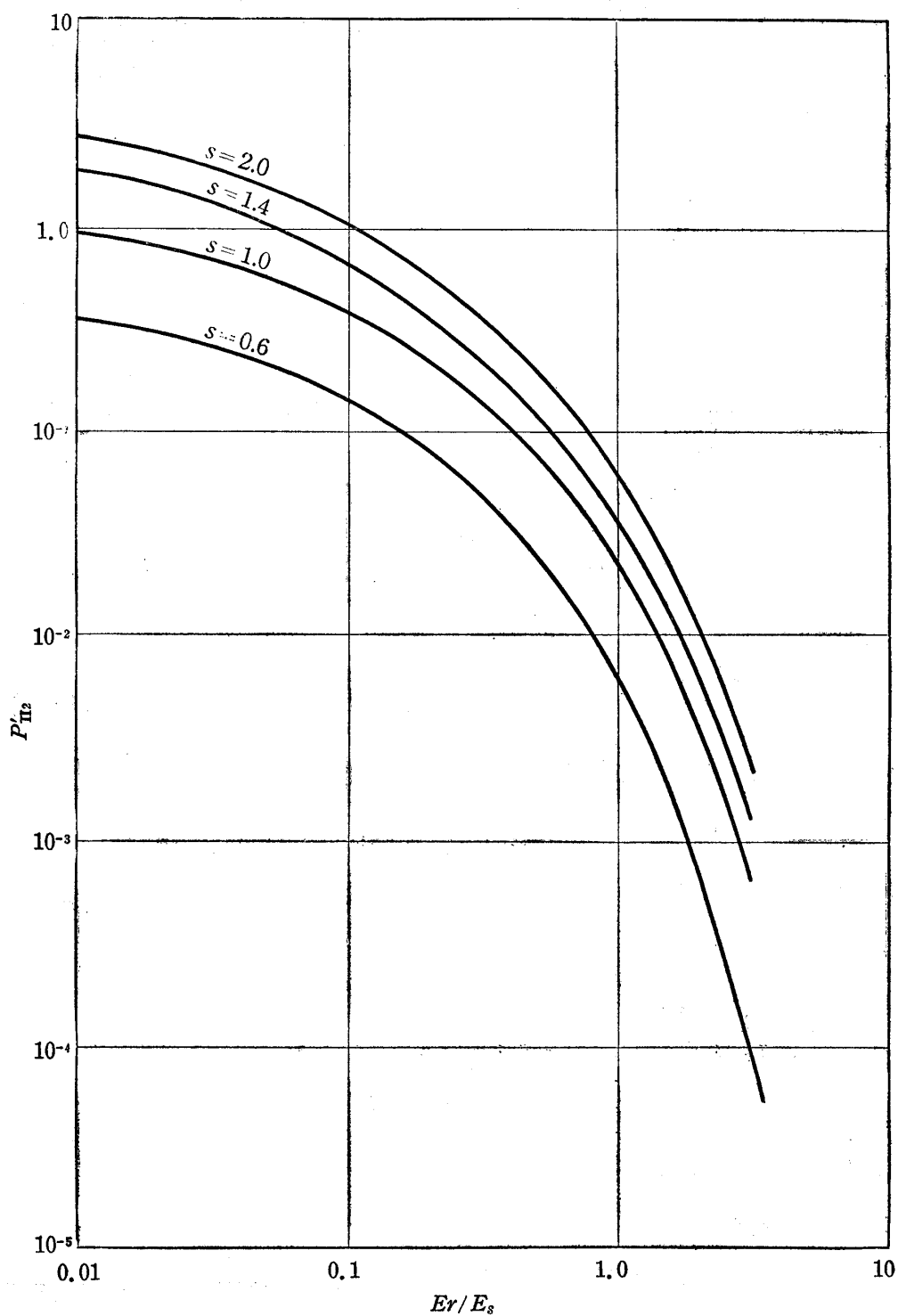
Fig. 1. Normalized integral structure functions, \left(\frac{Er}{E_s}\right)^{s-2} P'_{\Pi_2} , at a few different ages in the approximation A. (See Table 1, p. 113.)
