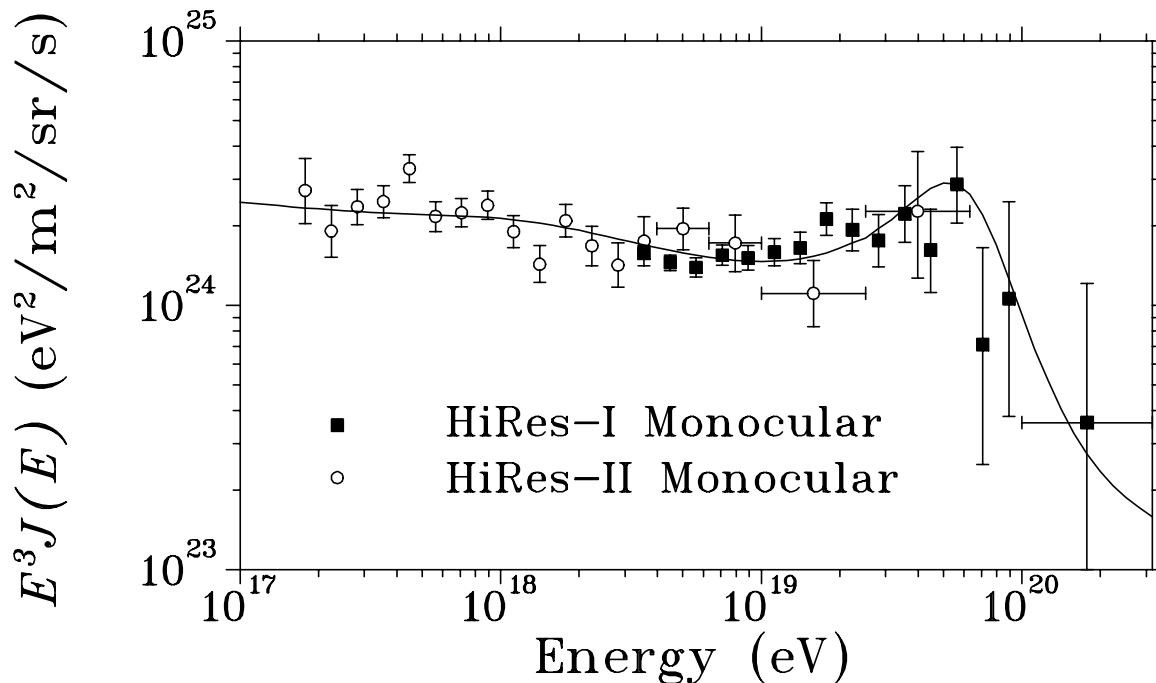
Combined HiRes I and II monocular spectra
