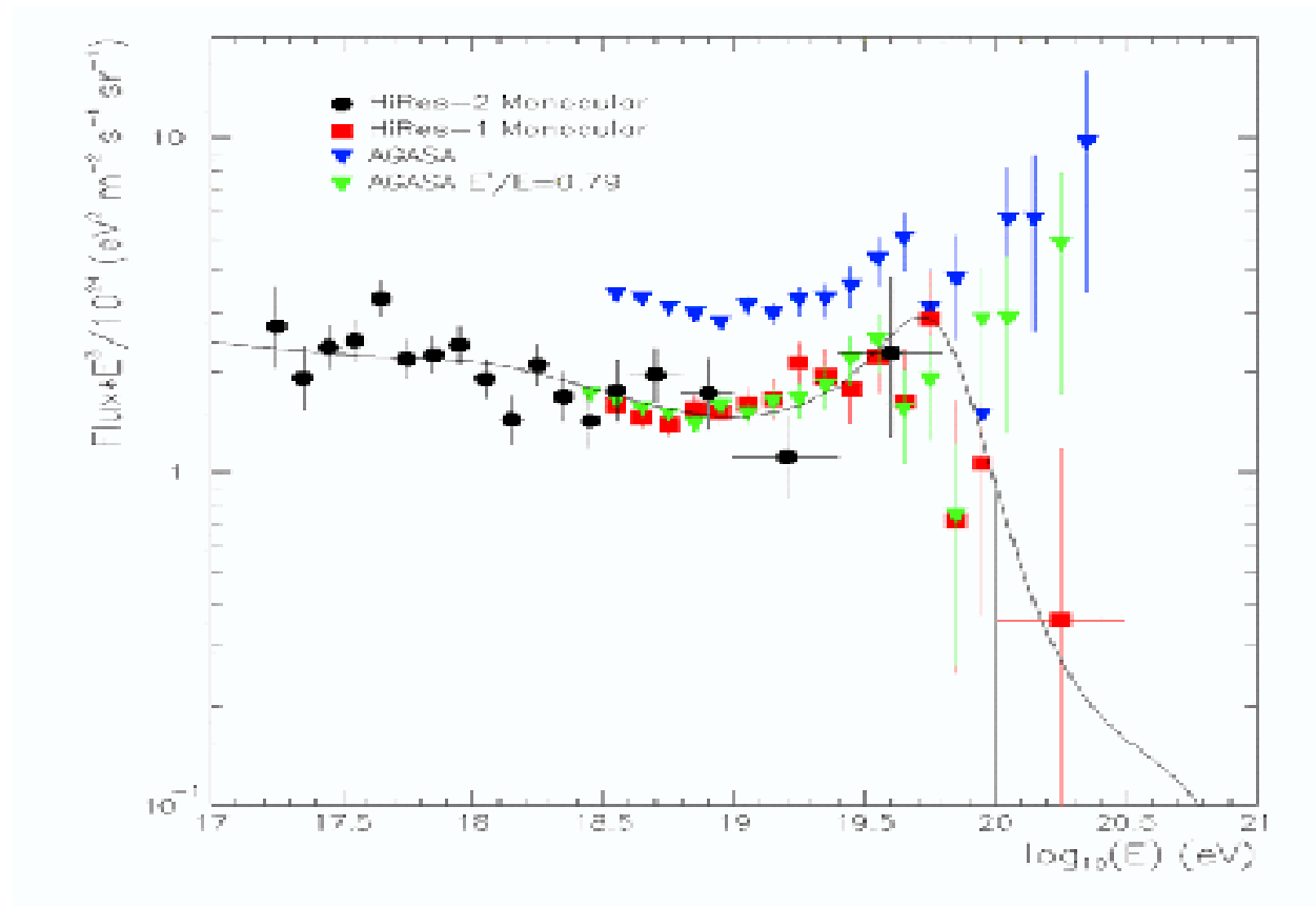
New HiRes data compared with AGASA
